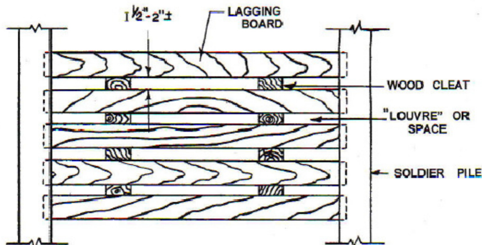
Figure 3: Elevation view of lagging members (Figure from FHWA Publication)
